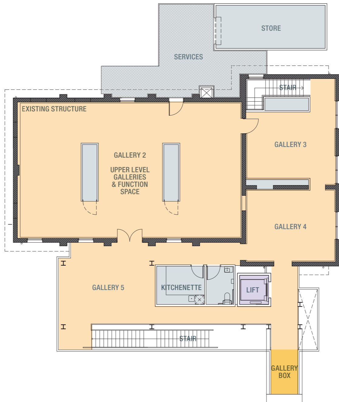
LEVEL 1 PLAN
