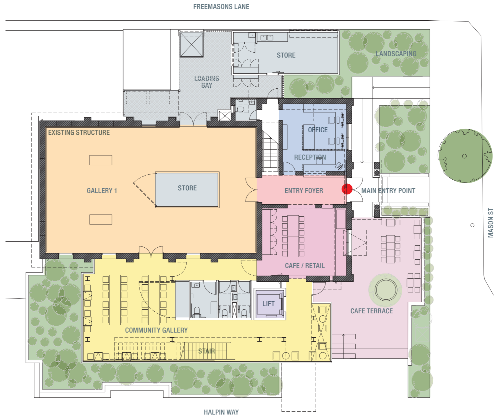
GROUND LEVEL PLAN
